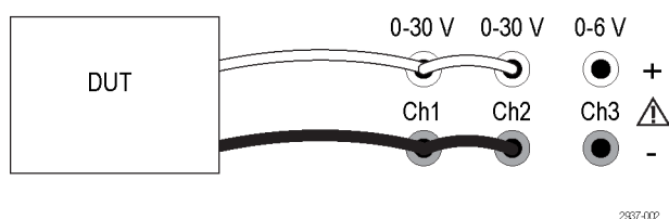
Figure 4: Parallel setup for model 2230-30-1 and device under test. Parallel setup for model 2220-30-1 is the same, but Channel 2 is on the far right.
