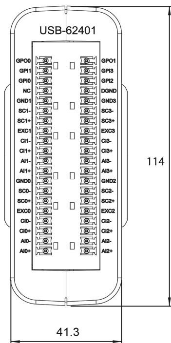
Figure 1-2: USB-62401 Module Rear View
