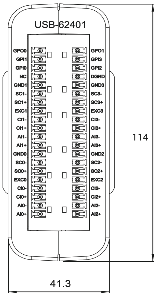
Figure 1-4: USB-62401 Module Front View
