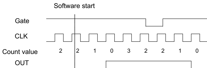
Figure 3-14: Mode 4-Single-Gated Pulse
