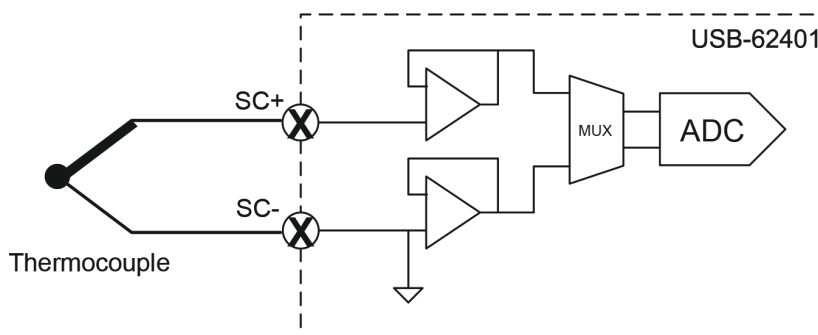
Figure 3-6: Thermocouple Connection
