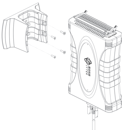
Figure 2-7: Module with Wall Mount Apparatus
