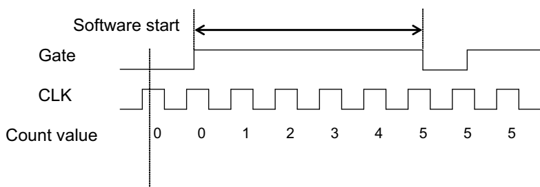
Figure 3-13: Mode 3-Single Pulse-Width Measurement
