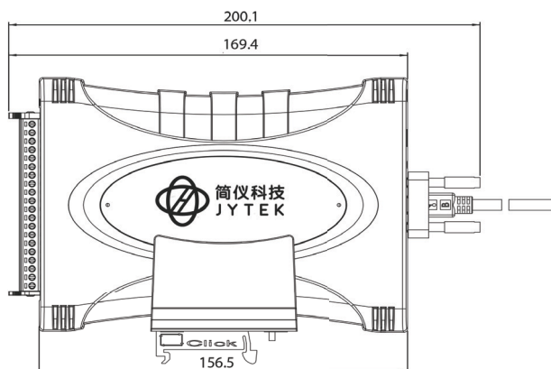
Figure 1-6: Module, Stand, & Wall Mount Kit Side View (w/ Connections)
