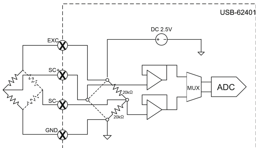
Figure 3-5: Full Bridge and Half Bridge Connection
