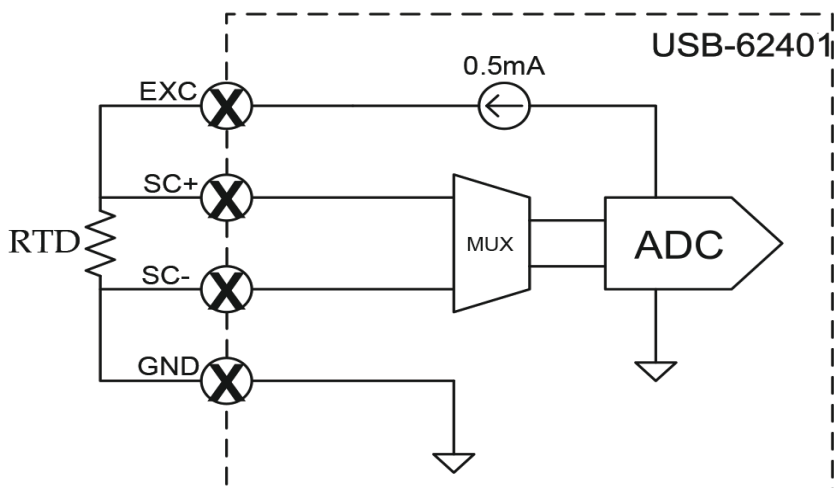
Figure 3-7: 4-Wire RTD Connection
