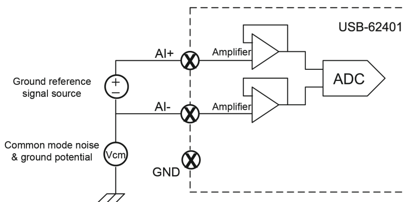
Figure 3-2: Ground-Referenced Source and Differential Input
