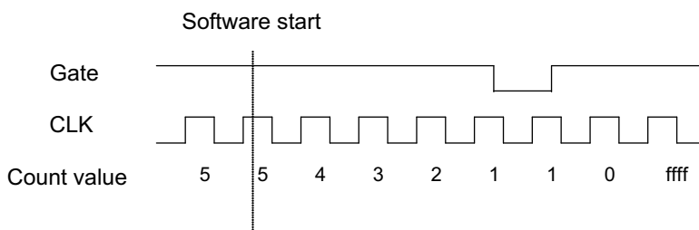
Figure 3-11: Mode 1-Simple Gated-Event Calculation
