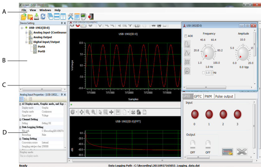
Figure 1-1: U-Test Interface
