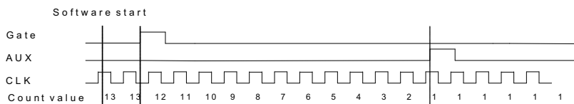
Figure 3-19: Mode 9-Edge Separation Measurement
