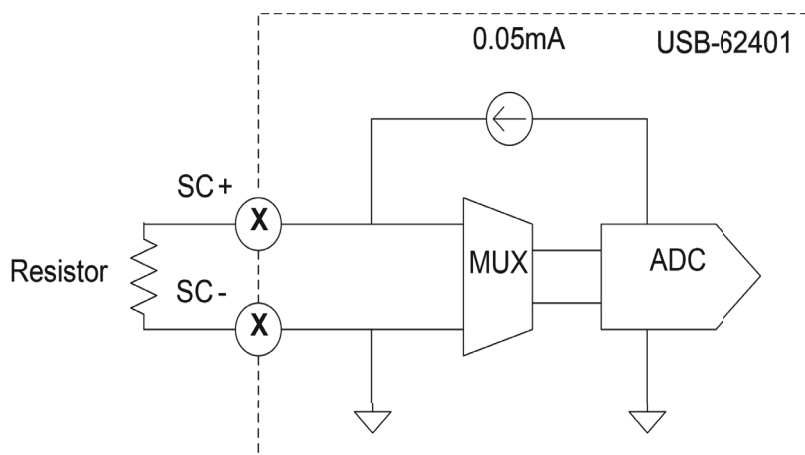
Figure 3-10: 2-Wire Resistance Connection
