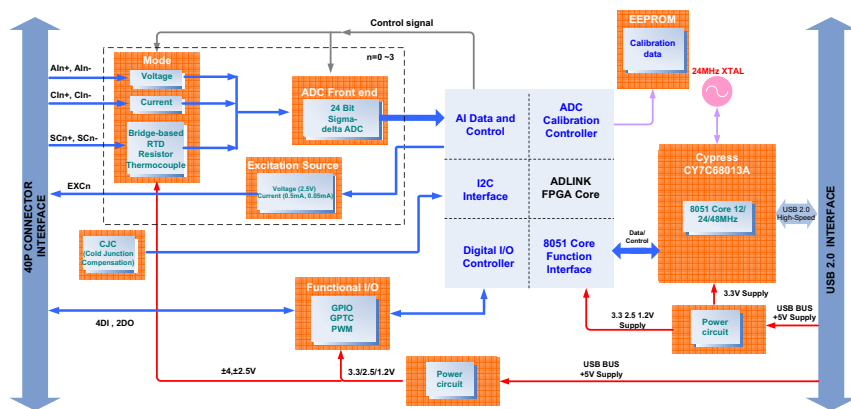
Figure 3-1: USB-62401 Functional Block Diagram
