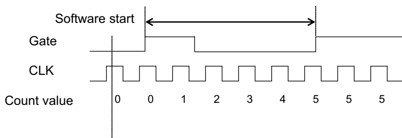
Figure 3-12: Mode 2-Single Period Measurement
