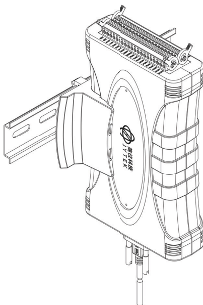
Figure 2-5: Module Rail-Mounted
