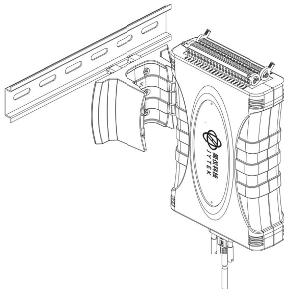
Figure 2-4: Module Pre-Rail Mounting
