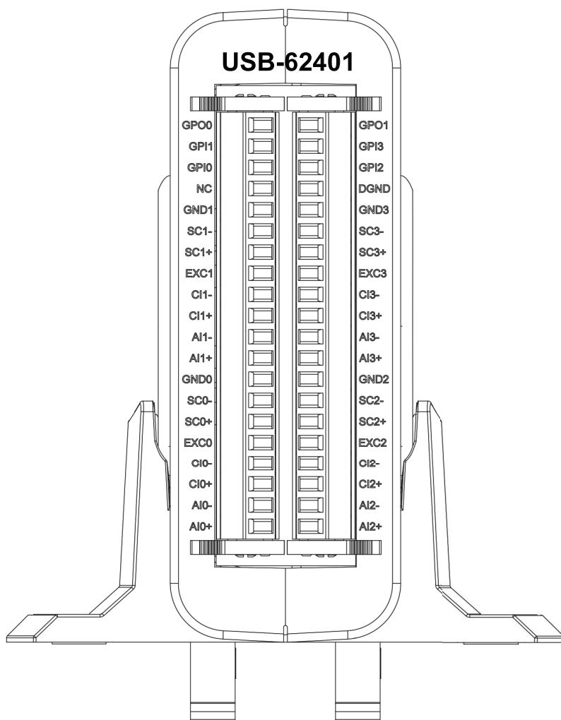
Figure 1-7: Module In Stand Front View
