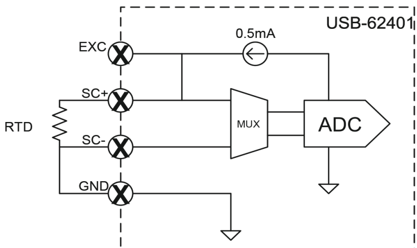
Figure 3-8: 3-Wire RTD Connection
