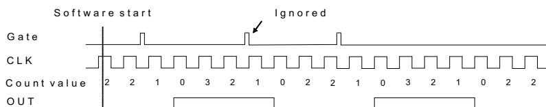
Figure 3-16: Mode 6-Re-Triggered Single Pulse
