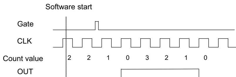
Figure 3-15: Mode 5-Single-Triggered Pulse
