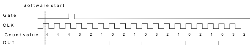
Figure 3-17: Mode 7-Single-Triggered Continuous Pulse
