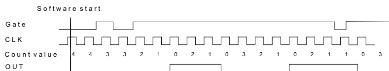
Figure 3-18: Mode 8-Continuous Gated Pulse
