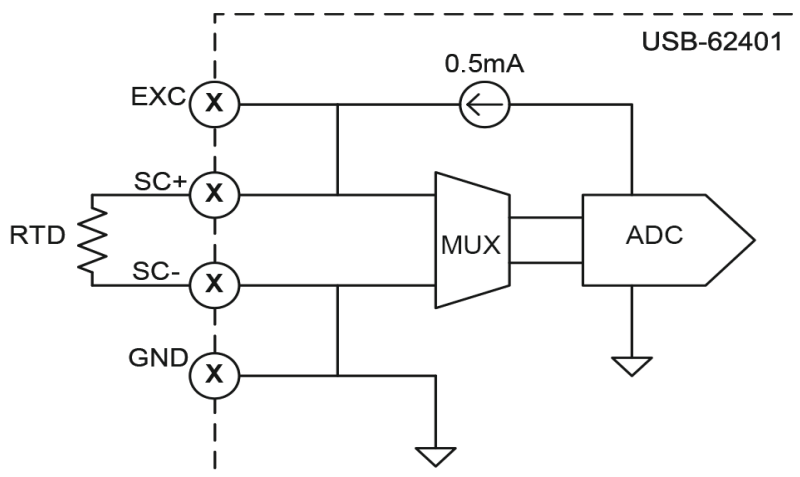
Figure 3-9: 2-wire RTD Connection
