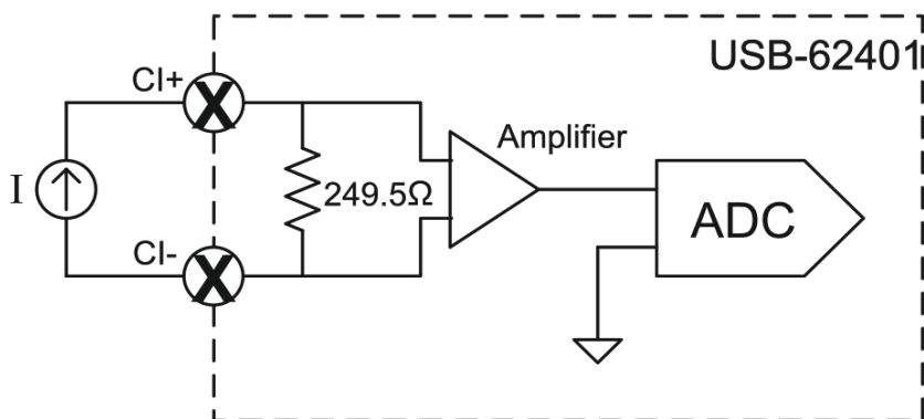
Figure 3-4: Current Source Connection
