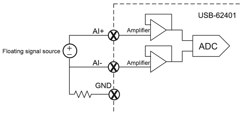
Figure 3-3: Floating Source and Differential Input
