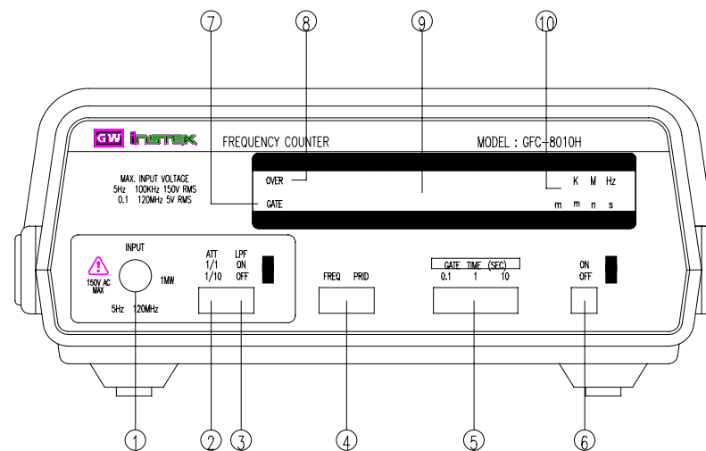
Fig. 1 Front panel
