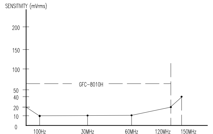
Fig. 5 Input Sensitivity Characteristic
