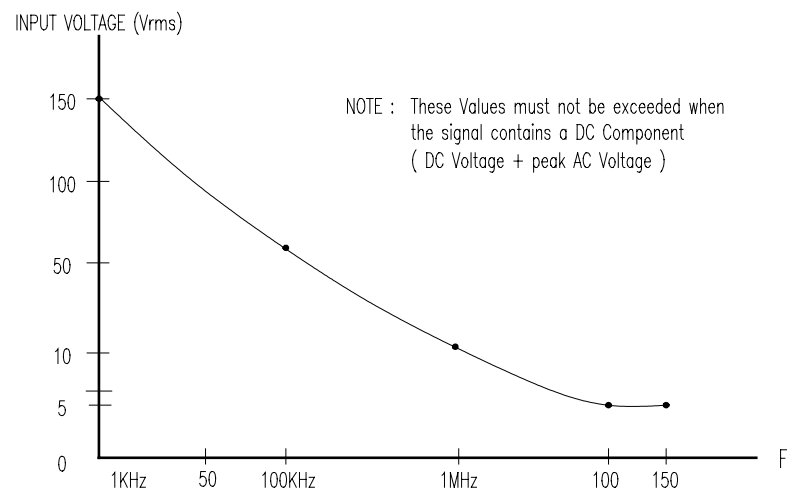
Fig. 6. Maximum Input Voltage-Frequency
