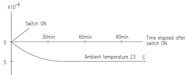
Fig. 9 Example of crystal oscillator rise characteristics
