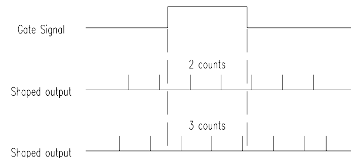
Fig. 7 \pm 1 count error
